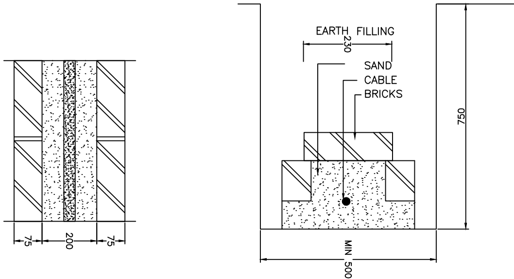
1 . FOR SINGLE CABLE OF OVERALL OUTER DIA UPTO 25 MM
