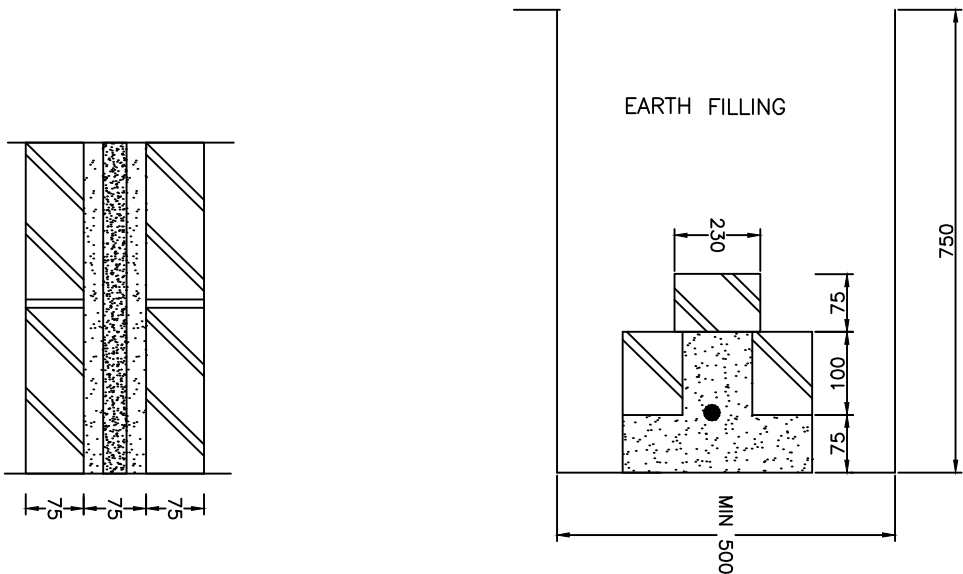
2. FOR SINGLE CABLE OF OVERALL OUTER DIA ABOVE 25 MM
