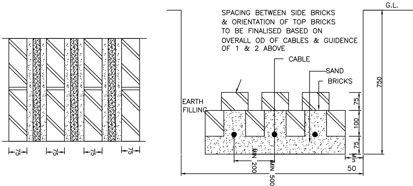
3. FOR GROUPING OF CABLE IN SAME TRENCH ( TYPICAL)
