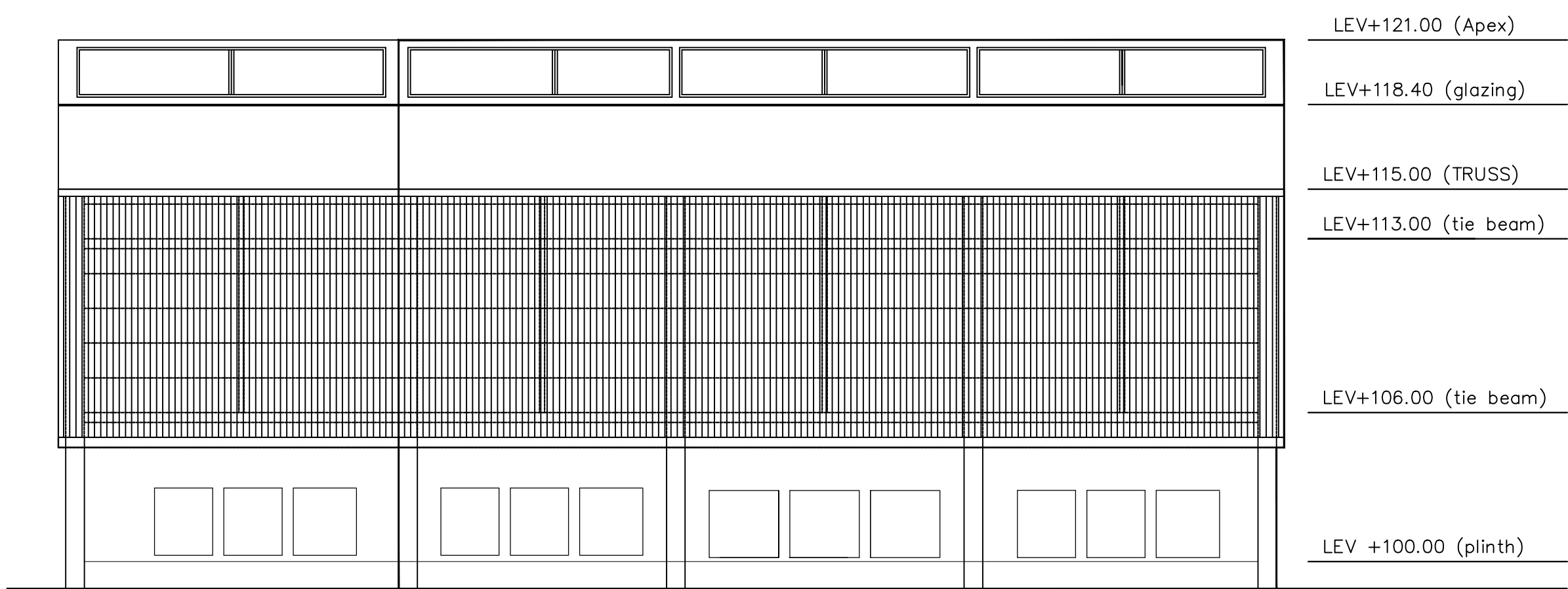
NORTH SIDE ELEVATION SCALE: 1:100
