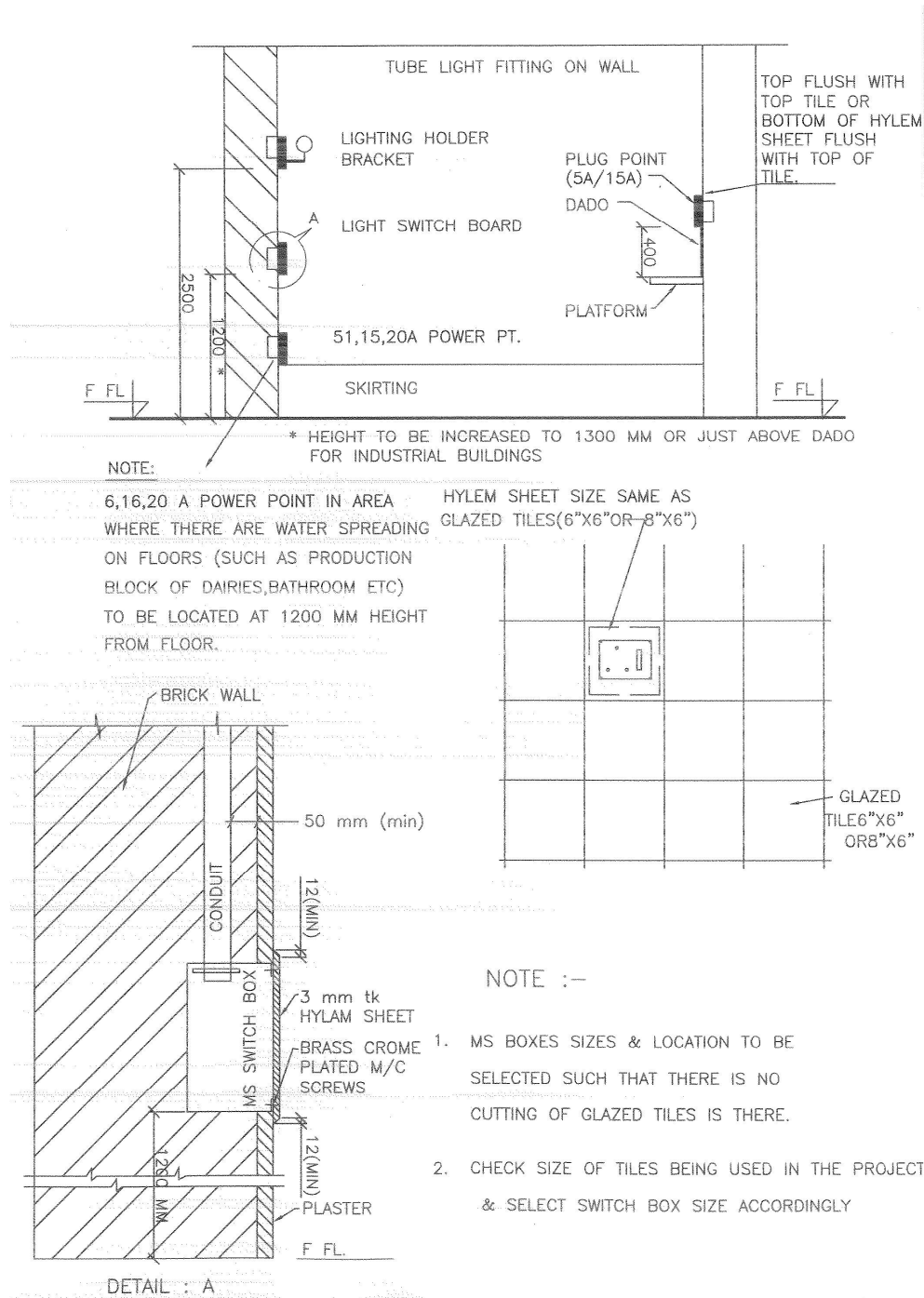
Fig-5, Installation tips for lighting Switch board.
