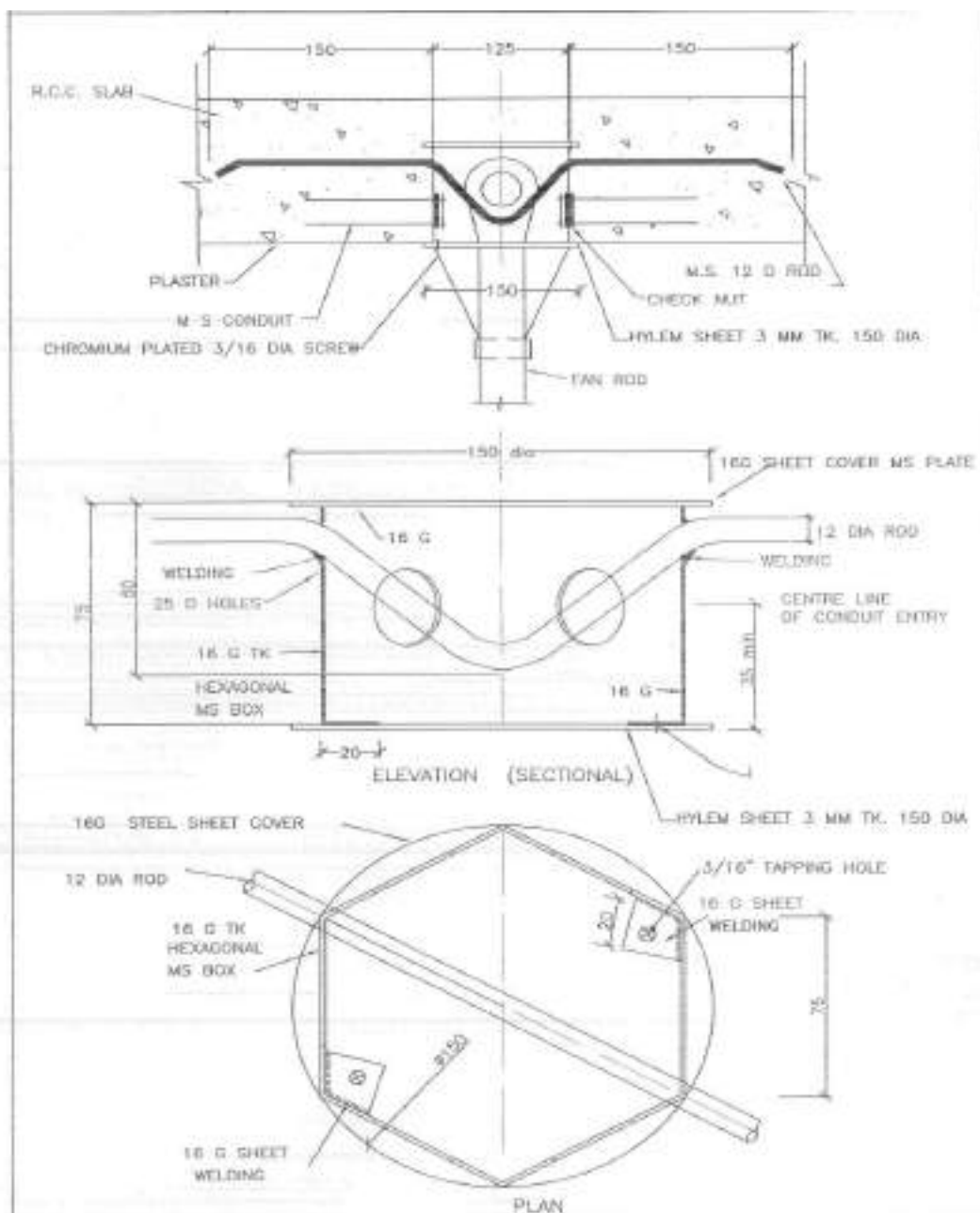
Fig-3, Outlet box and installation for ceiling fan.
