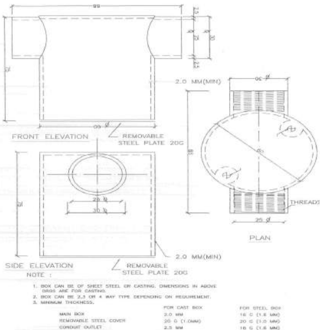
Fig– 1A, Details of outlet box for installation of light fitting on Slab.
