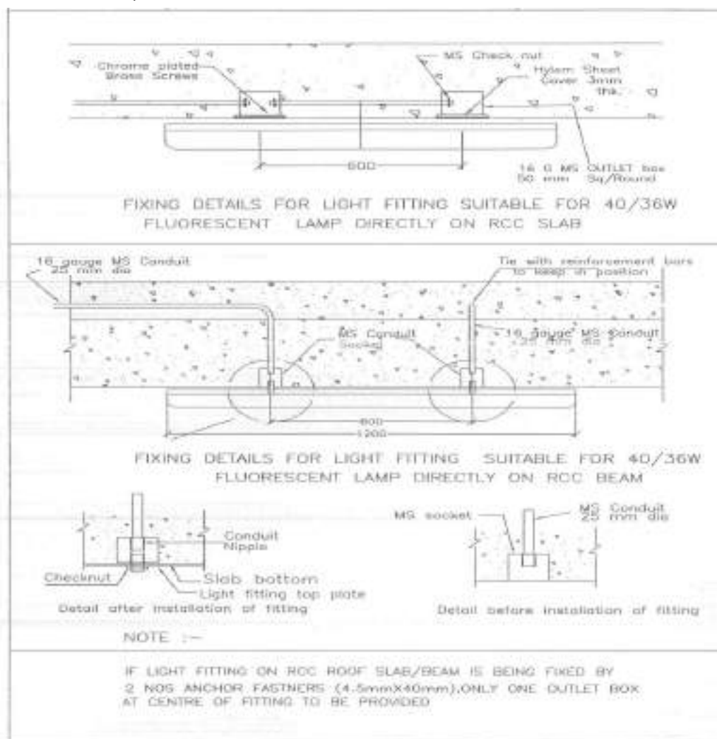
Fig – 2, Fixing details of Fluorescent light fitting.
